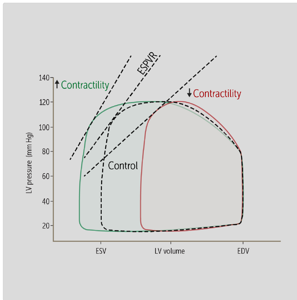
Figure 7 Effects of contractility on the PV loop- altered ESV, and SV
