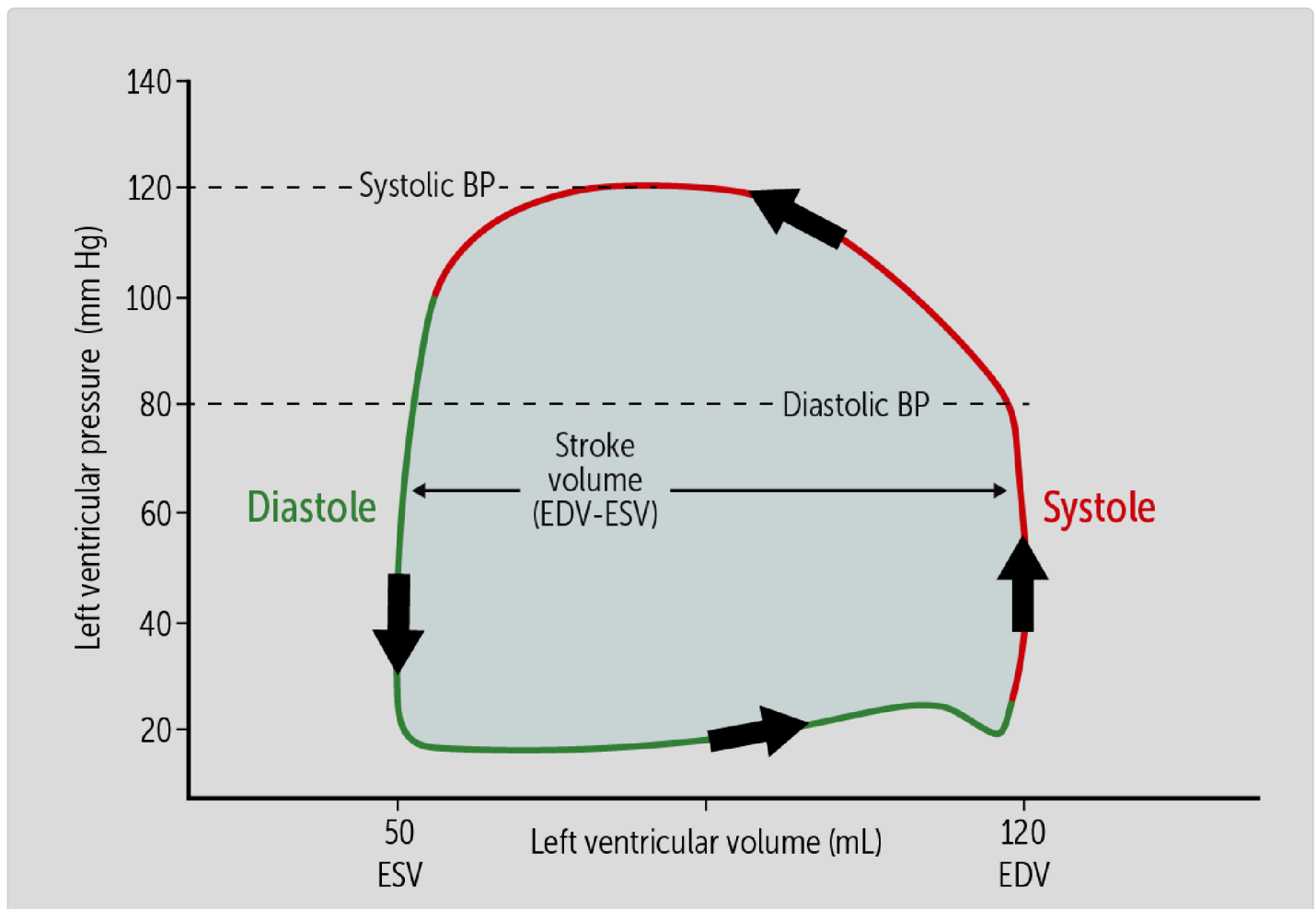
Figure 4. Blood pressures, stroke volume (arrow) and stroke work (blue shading) related to the PV loop
