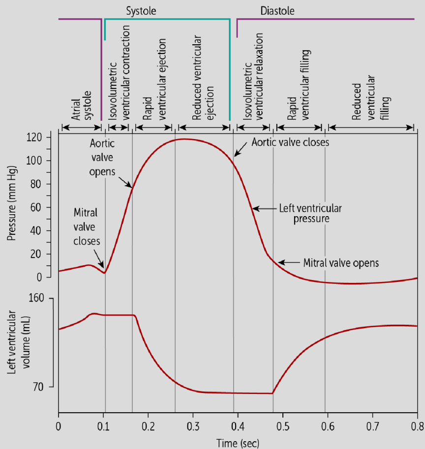
Figure 2 Pressure and volume changes in the cardiac cycle
