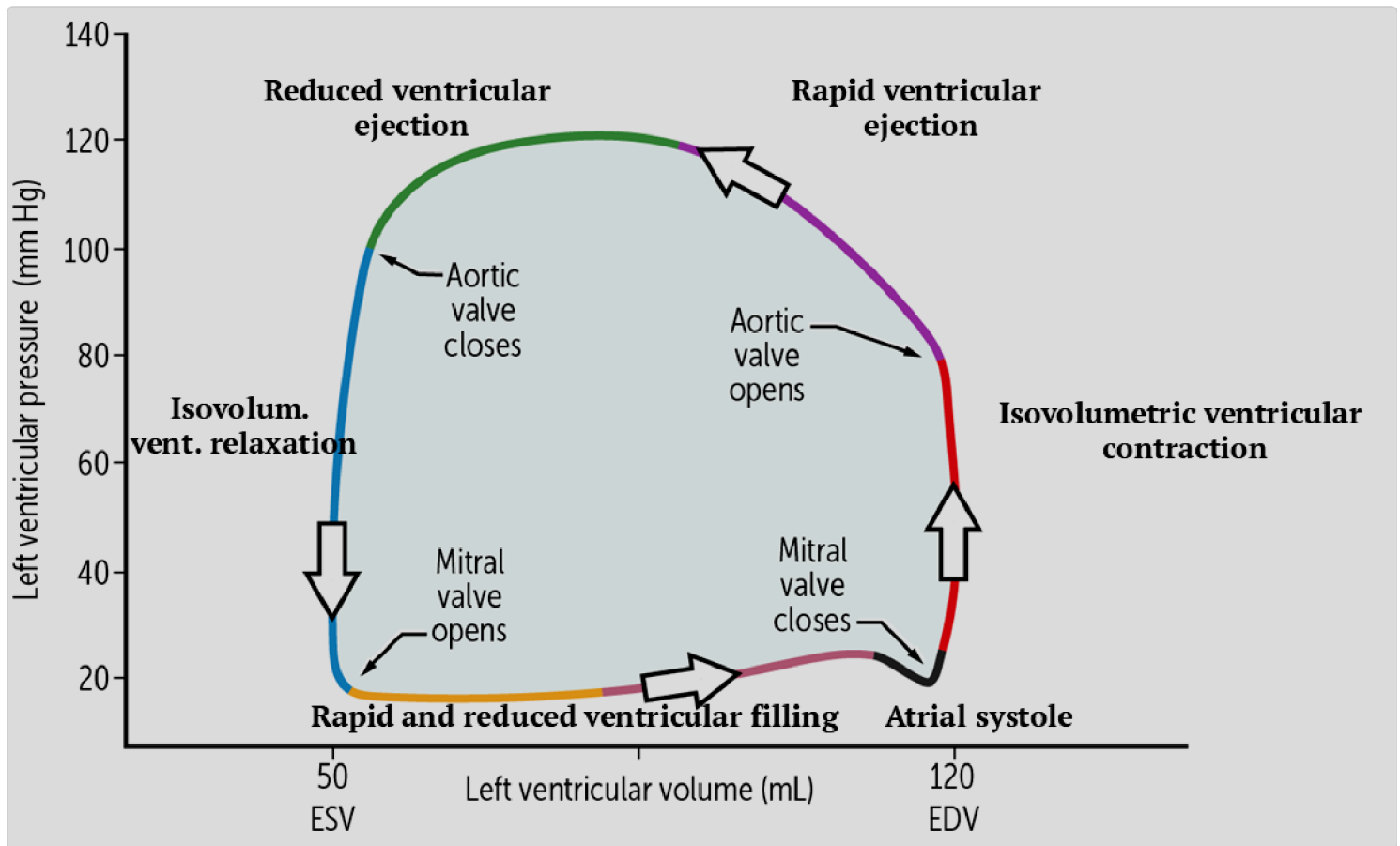
Figure 3 Normal left ventricle pressure-volume loop (labelled with cardiac cycle phases)
