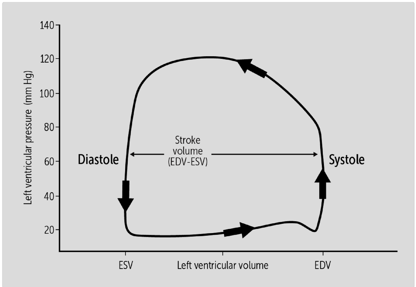
Figure 1 A basic left ventricle pressure-volume loop
