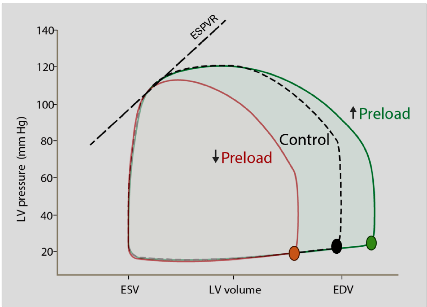
Figure 5 Effects of preload on the PV loop- altered EDV and SV
