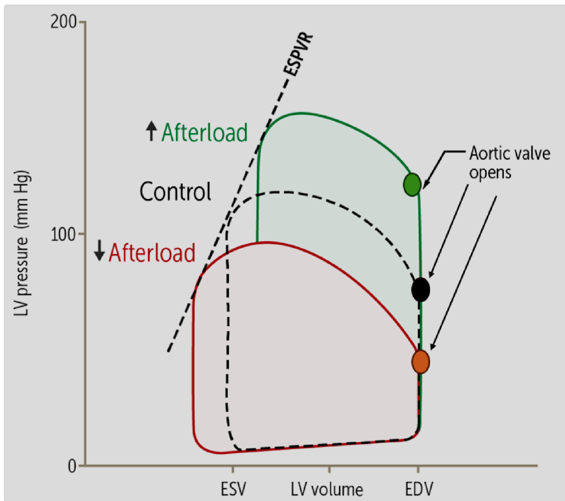
Figure 6 Effects of afterload on the PV loop- altered ESV, and SV
